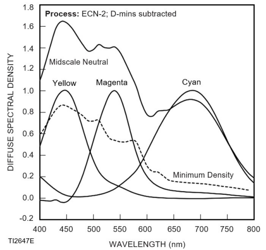
Spectral Dye Density Curves
